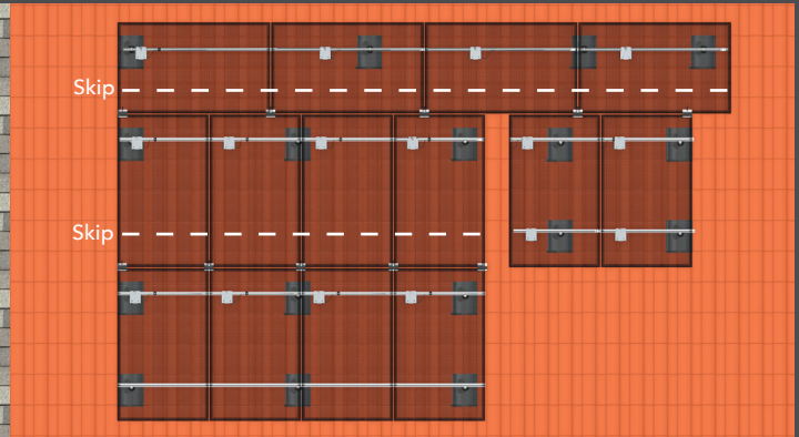
Example of Tile Roof Array
